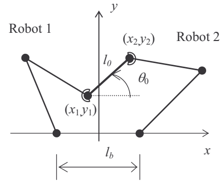
Fig. 1. Two 2R cooperating robots for the manipulation of an object with length l_0 and orientation \theta_0 .
