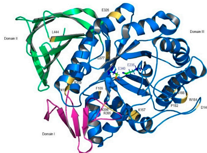
Figure 1. Location of GlcCerase missense mutations considered in this study presented in a solid ribbon model. Domain I is shown in pink, domain II is in green, and domain III is shown in blue. Mutations are identified in yellow. Active site residues (E235 and E340, in blue letters) are shown as ball-and-stick model, with different colors.
