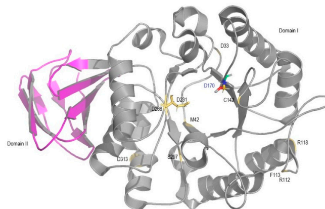
Figure 2. Location of \alpha -GAL missense mutations considered in this study presented in a solid ribbon model. Domain I is shown in grey and domain II is shown in pink. Mutations are identified in yellow, and active site residues (D170 and D231, the non-mutated active site residue in blue letters) are shown as ball-and-stick model, with different colors.
