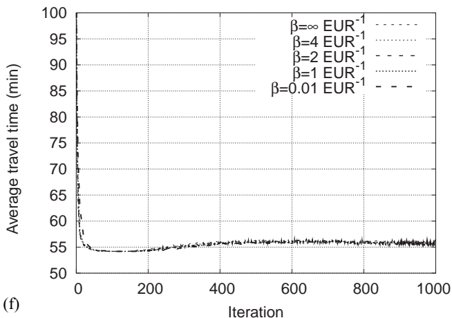
Figure 3.5.11 Relaxation of scores and travel times for the Routes Only scenario, comparing the relaxation behaviour with varying \beta values. These plots display the average values of the score (left) and travel time (right) collected over the entire population of agents during each iteration.
