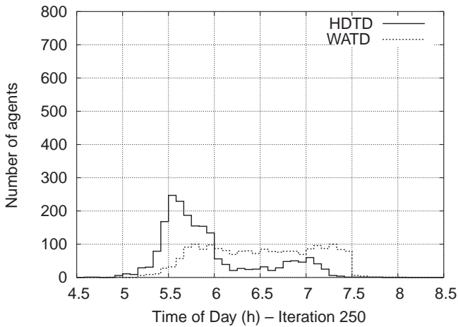
Figure 3.5.9 Histograms showing HDTD and WATD for the Times Only scenario, after relaxation (250 iterations). The histograms are taken over five minute time-bins.
