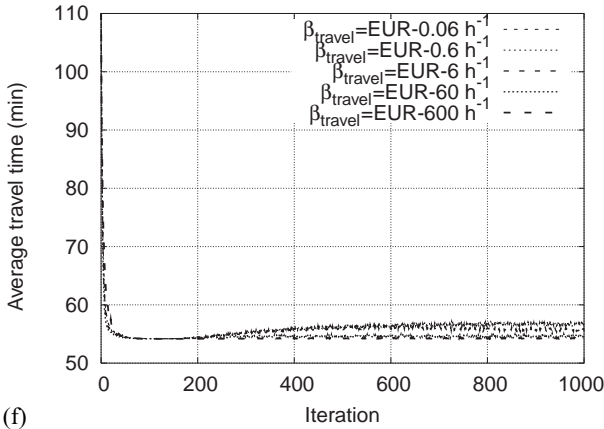
Figure 3.5.12 Relaxation of scores and travel times for the different scenarios, comparing the relaxation behaviour with varying \beta_{\text{travel}} values. These plots display the average values of the score (left) and travel time (right) collected over the entire population of agents during each iteration. For better comparison of the relaxation rate, we shift the average score curve for \beta_{\text{travel}} = \text{€-600h} up by \text{€500} .
