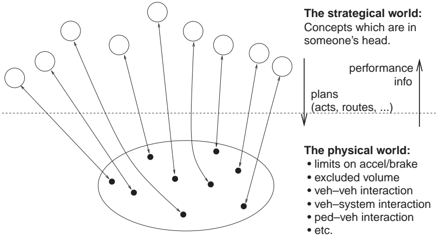
Figure 3.5.1 Physical and strategic layers of the framework.
