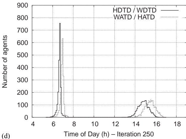
Figure 3.5.7 Histograms showing home departure time distribution (HDTD), work arrival time distribution (WATD), work departure time distribution (WDTD), and home arrival time distribution (HATD) of the three scenarios, before and after relaxation (250 iterations). The histograms are taken over five minute time-bins. For clarity, the range stops at 900 vehicles, though some of the initial departure peaks are above this value; these peaks are labelled with their actual values.
