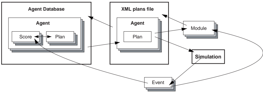
Figure 3.5.3 Components and data flow in the framework.
