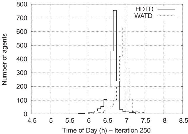
Figure 3.5.10 Histograms showing HDTD and WATD for the Routes and Times scenario, after relaxation (250 iterations). The histograms are taken over five minute time-bins.
