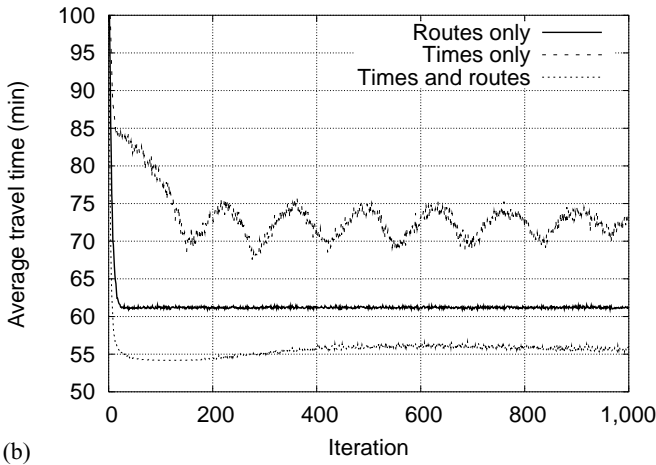
Figure 3.5.6 Relaxation of score and travel times for all three scenarios of the baseline case. These plots display the average values of the (a) score and (b) travel time collected over the entire population of agents during each iteration.
