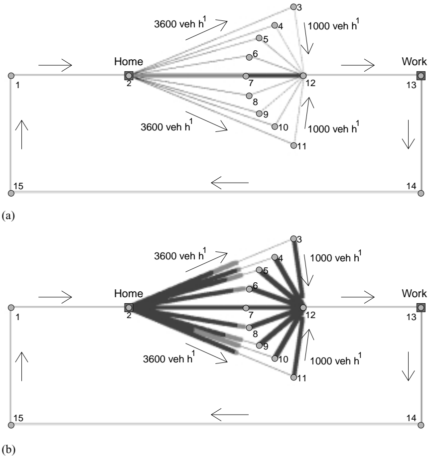
Figure 3.5.5 Diagram of the testing network overlaid onto example snapshots of the Routes Only scenario at 06.08 am, (a) before and (b) after many iterations of route replanning. After replanning, the agents have spread onto the different available routes between home and work. Link capacities are 36 000 veh/h except where indicated (the nine route options are identical).
