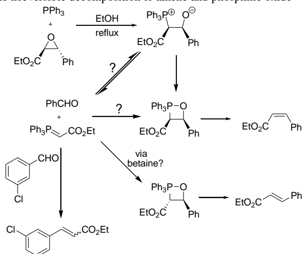
Scheme 4. Independent betaine generation by nucleophilic cleavage of epoxide with phosphine. 54 Reversal of OPAs derived from stabilised ylides to Wittig starting materials had not been unequivocally ruled out 60 at the time of the formulation of the betaine mechanism, so would have been considered in principle to be a possibility, as indicated in this scheme.
