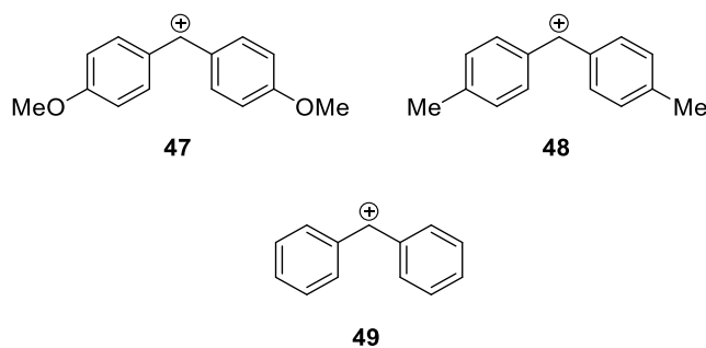
Chart 2. Benzhydrylium ions 47 - 49 .
