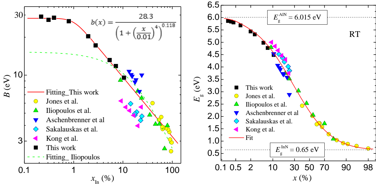
Figure 3-18 InAlN bowing parameter and band gap with their best fit (using b(x) equation) in full range of In contents, in combination with other previously reported data [154, 155, 157, 159, 321].
