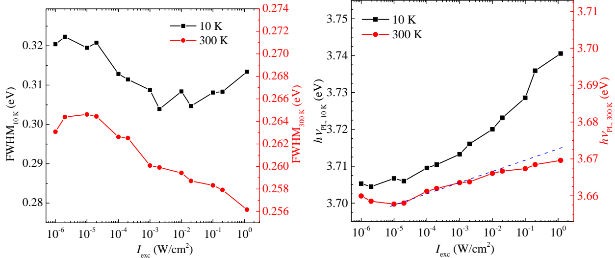
Figure 4-11 Emission peak energy and full width at half maximum (FWHM) as a function of excitation power density for the InAlN/AlGaN MQWs at 10 K and 300 K.
