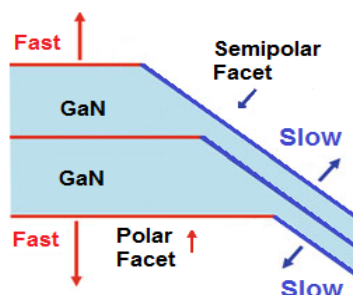
Figure 5-9. Schematic diagram of growth rate on polar and semipolar facets.
