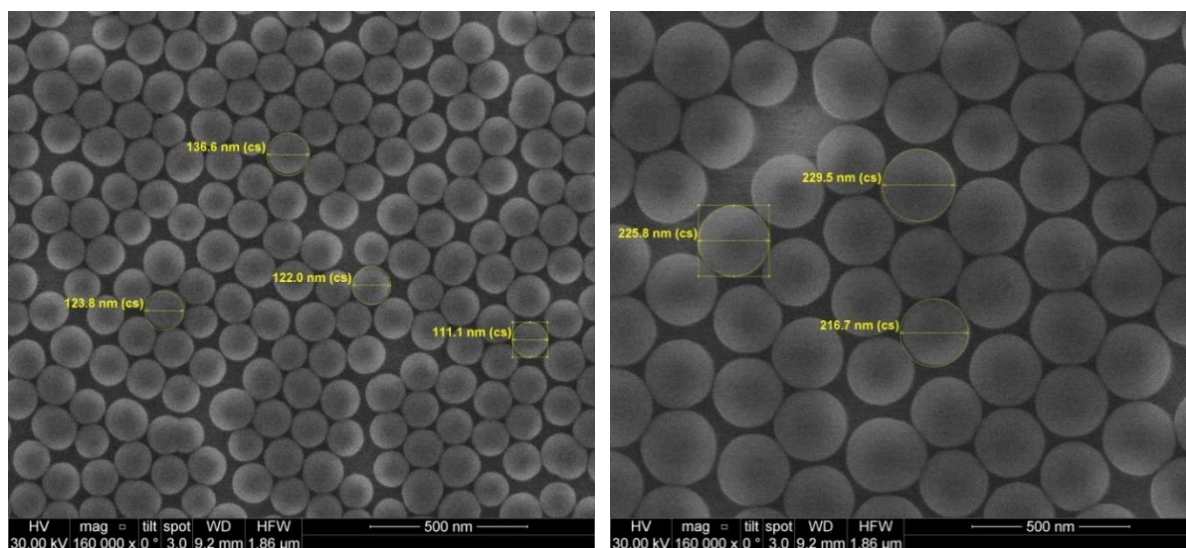
Figure 5-2. SEM top image of silica nanospheres GaN/Sapphire template at two nominal sizes of 120 nm and 210 nm.
