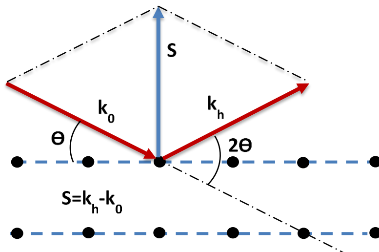
Figure 2-14. Schematic illustration of relationship between the incident ( k_0 ), diffracted ( k_h ) and scattering ( S ) vectors with respect to the crystal.
