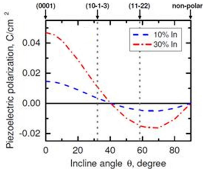
Figure 1-13 Calculated polarization charge density for In_{0.1}Ga_{0.9}N and In_{0.3}Ga_{0.7}N versus incline angle [8].
