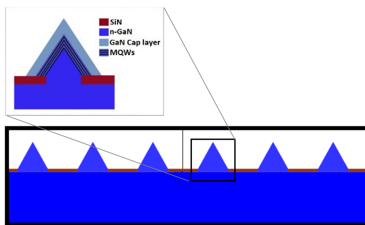
Figure 5-15. Growth Schematic
