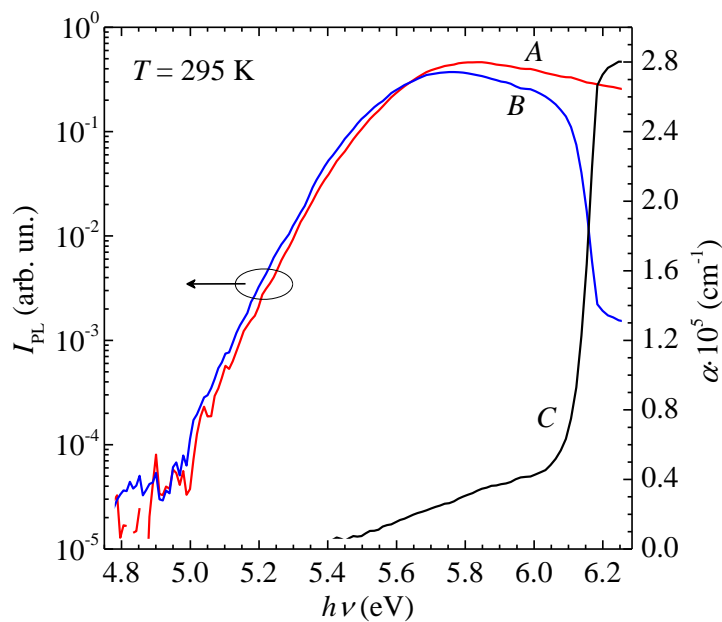
Figure 3-15 PLE spectra of uncapped (curve A) and AlN-capped (curve B) In_{0.019}Al_{0.981}N layers as well as the resulting absorption spectrum of AlN (curve C) determined from Equation 3-8.
