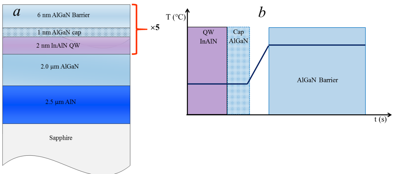
Figure 4-1 Schematic illustration of growth structure (a) and temperature profile during growth (b) of InAlN/AlGaN MQWs.
