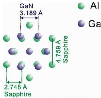
Figure 2-11 Schematic top view of the epitaxial relationship between GaN (0001) and Al_2O_3 (0001) [233].
