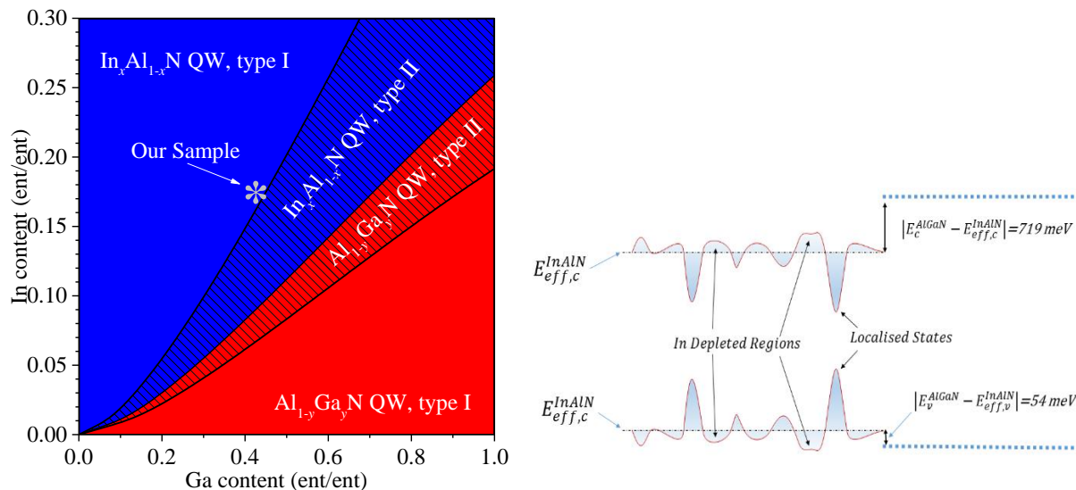
Figure 4-14 a: Composition dependent band offset of InAlN and AlGaN alloys, b: Schematic band structure of In_{0.18}Al_{0.82}N/Al_{0.59}Ga_{0.41}N and an indication of localised states and In depletion regions.
