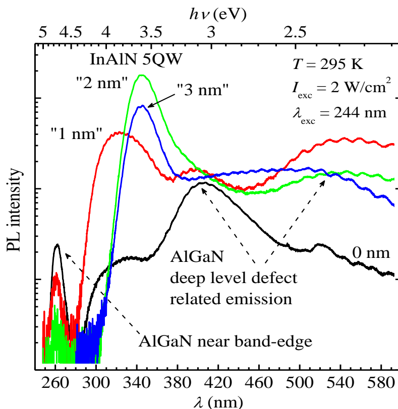
Figure 4-2 RT PL spectra of InAlN/AlGaN 5QW structures with different nominal QW cap layer thicknesses [187].
