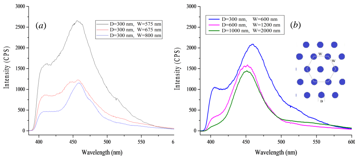
Figure 5-28 \mu -PL spectroscopy of nano-structured LED. The effects of pitch (a) and size (b).
