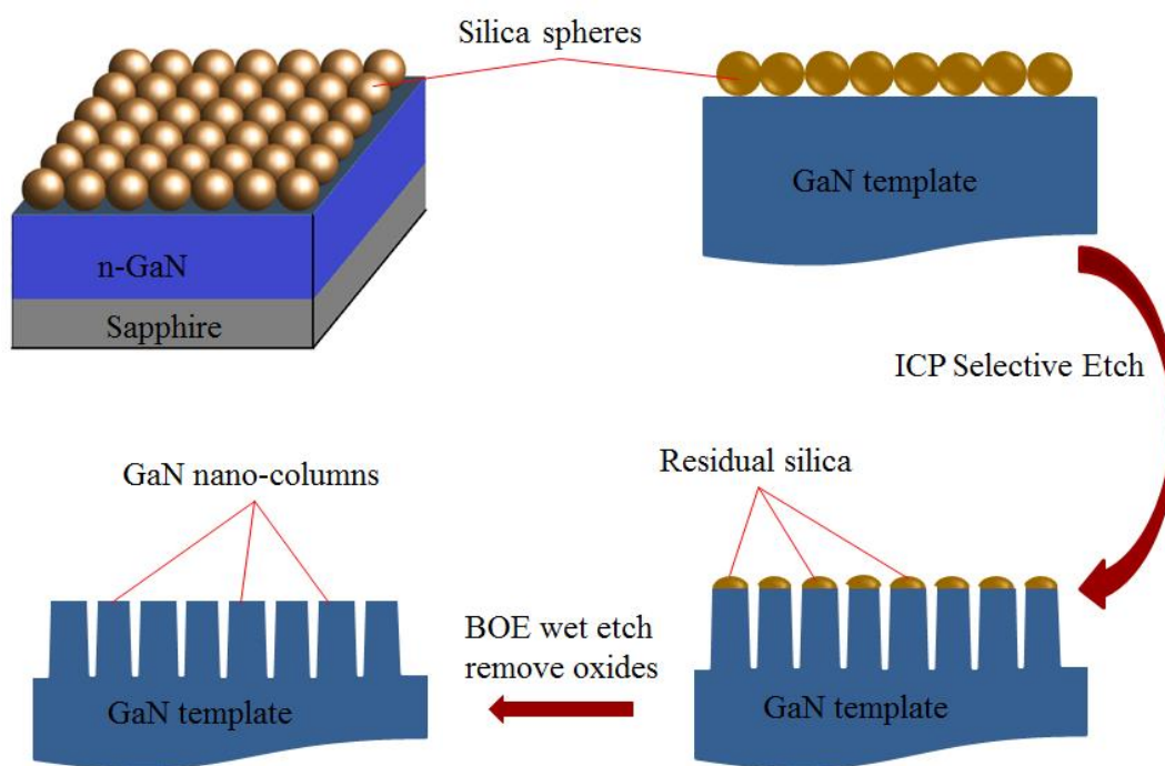
Figure 5-3. Schematically shown experimental method to fabricate nano-columns.
