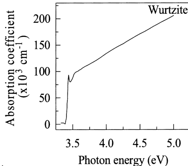
Figure 1-16 The room temperature absorption coefficient versus photon energy for wurtzite GaN grown on sapphire [170].
