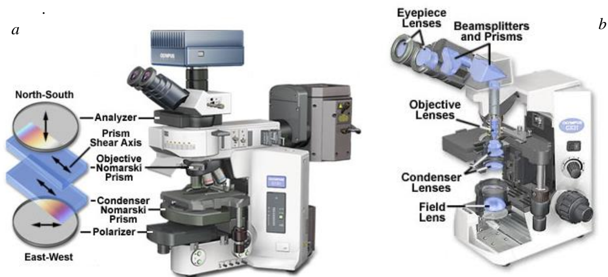
Figure 2-18. Typical Nomarski microscope configuration (a) and locations of the lenses and optical paths [253]
