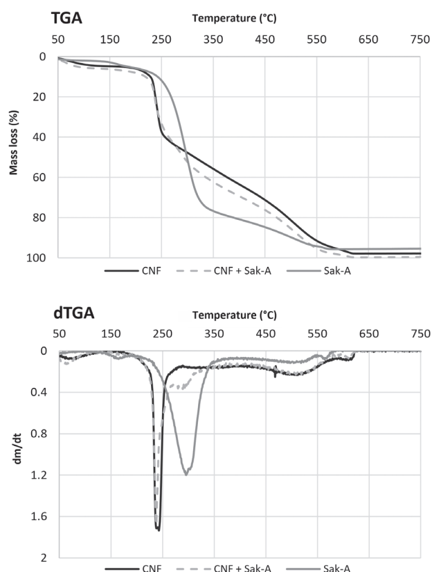
Figure 4. Thermogravimetric analysis of materials prepared employing cellulose nanofiber (CNF) only and CNF–sakacin-A: a, original unit; b, first derivative. The behavior of an enriched sakacin-A solution at the same concentration employed is also reported.
