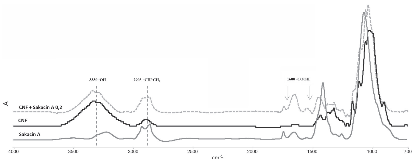
Figure 3. FTIR spectra of materials prepared employing cellulose nanofiber (CNF) only and CNF–sakacin-A; spectrum of the sakacin-A enriched extract in the same condition is also reported.
