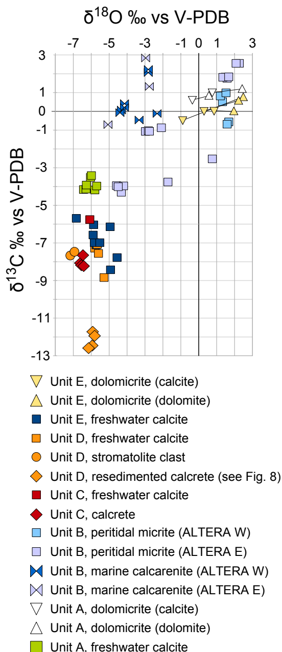
FIGURE 7 | Stable isotope composition of the carbonate deposits in the study area (see text for description).
