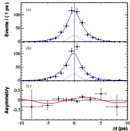
FIG. 2 (color online). Projections onto \Delta t for \eta'K_S^0 of the data (points with error bars), fit function (solid line), and background function (dashed line), for (a) B^0 and (b) \bar{B}^0 tagged events, and (c) the asymmetry between B^0 and \bar{B}^0 tags.
