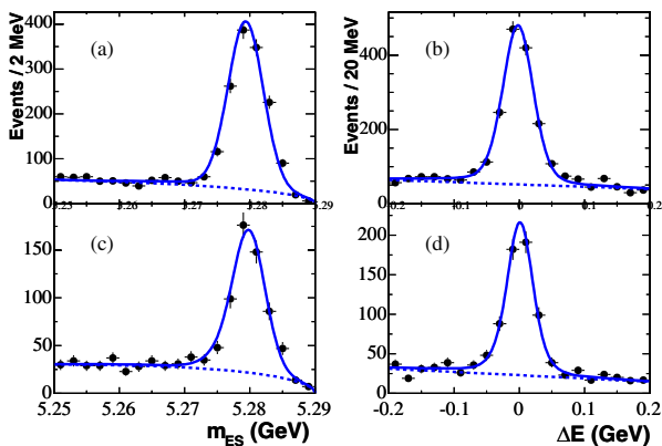
FIG. 1 (color online). The B candidate m_{\text{ES}} and \Delta E projections for \eta'K^+ (a),(b) and \eta'K_S^0 (c),(d). Points with error bars represent the data, the solid line the fit function, and the dashed line its background component.
