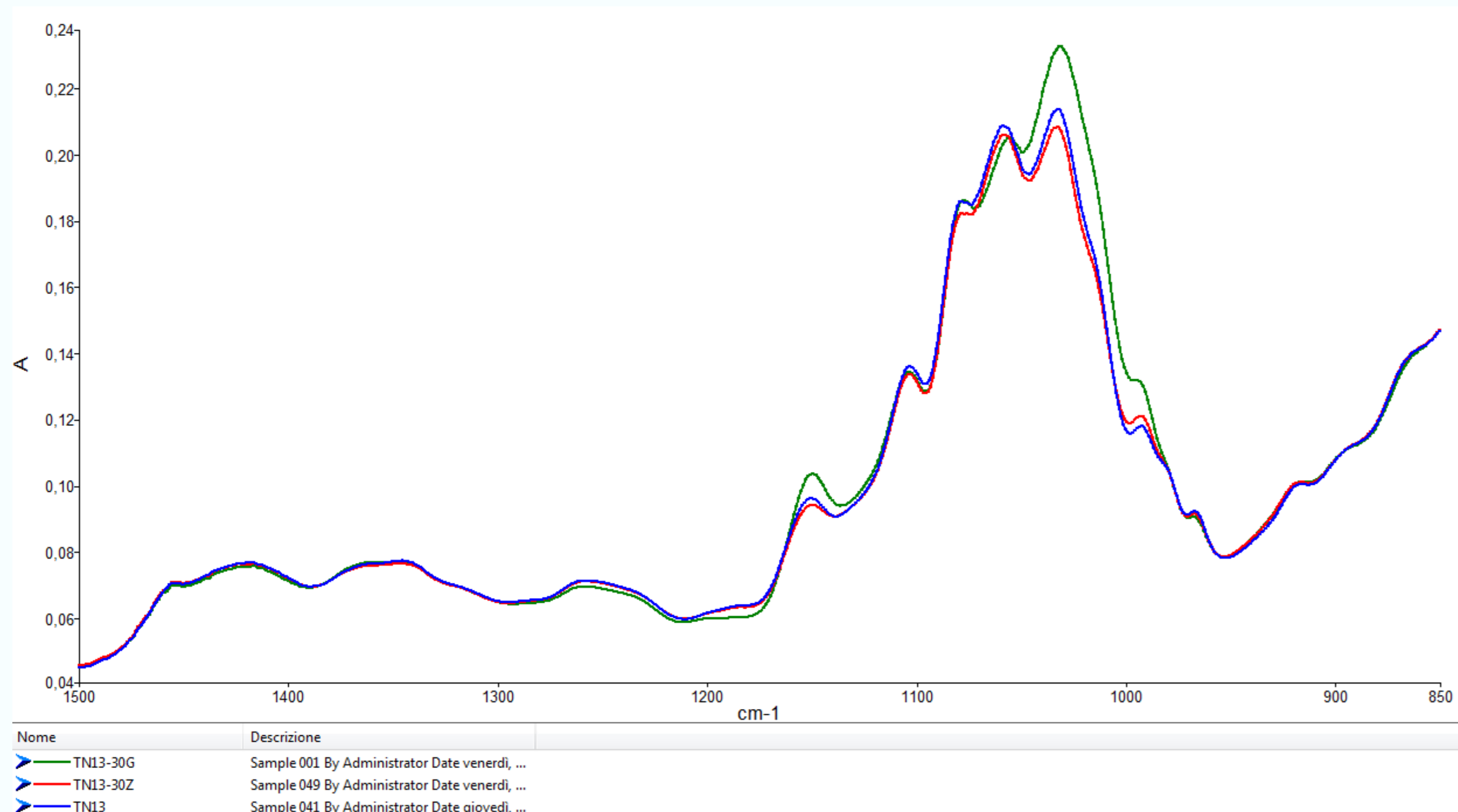
Figure 1: FTIR-ATR spectra of adulterated and non adulterated honey
