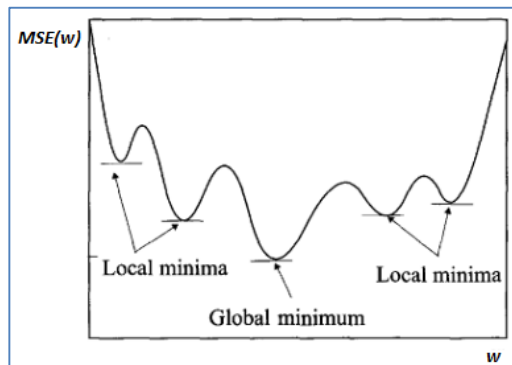
Figure 13 Global minimum and local minimums, one-dimensional example. Source: (Gupta 2003: 162).
