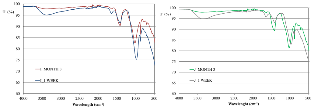
Figure 5. Comparison of FT-IR spectra for 3 months and 1 week of a) I specimen b) J specimen.
