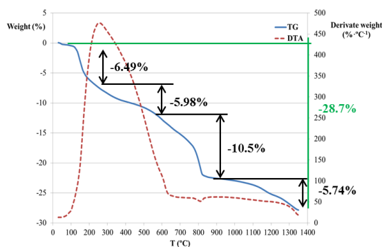
Figure 1. TGA result for the WBA raw material.
