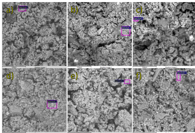
Figure 3. Micrographies for different geopolymeric samples a) I and b) J after 15 days of curing; c) I and d) J after 2 months of curing; e) I and f) J after 3 months of curing.
