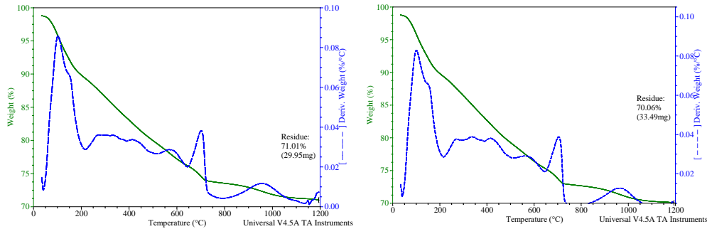
Figure 4. TGA results for the I and J formulations at 3 months of curing.
