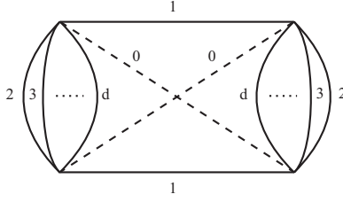
Figure 2: A (d + 1) -colored graph representing the (d - 2) -th suspension of \mathbb{R}P^2
