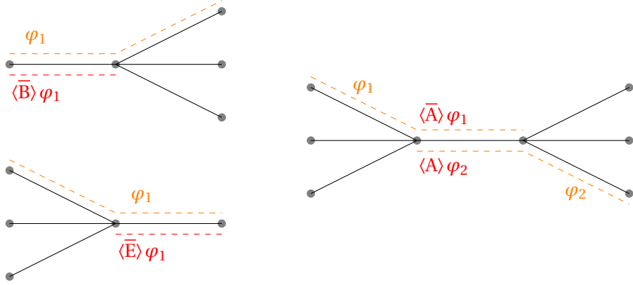
Figure 1: State-based semantic variant \text{HS}_{\text{st}} : past and future are branching.
