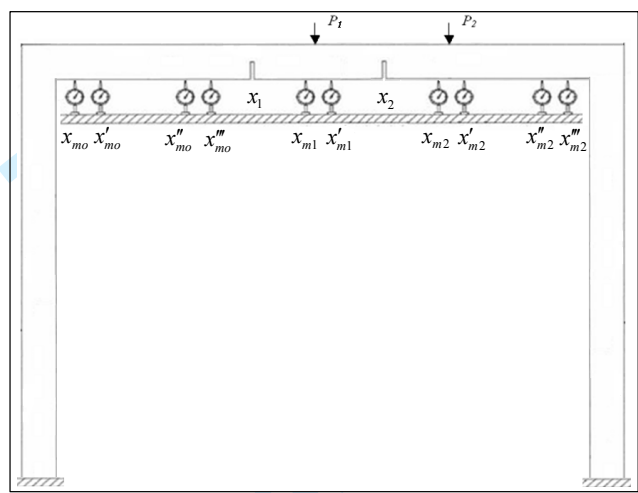
Fig. 9 A frame with two concentrated cracks
