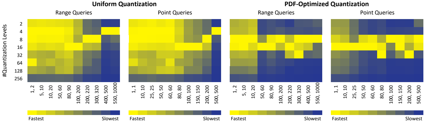
Fig. 9: Uniform and PDF-optimized scalar quantization parameter setup.
