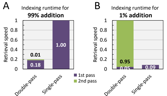
Fig. 11: Benchmarking single and double pass indexing algorithms for two scenarios.
