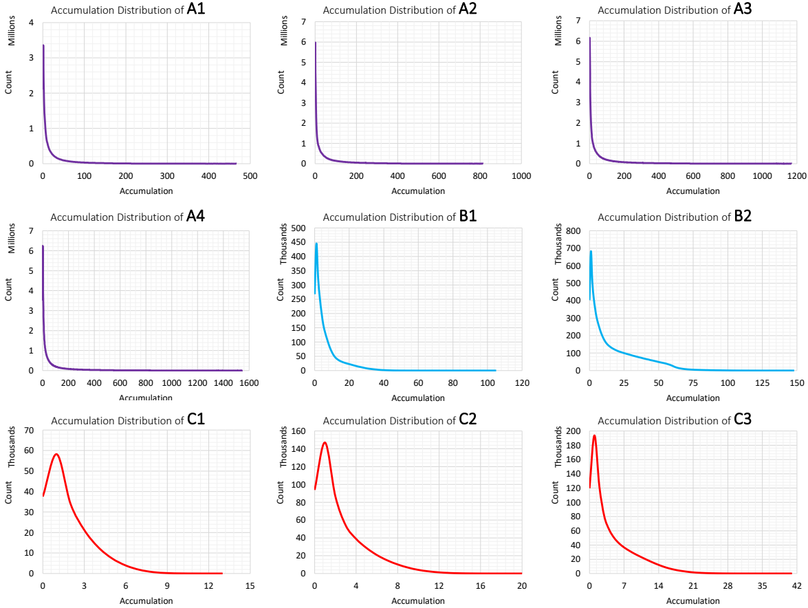
Fig. 14: Accumulation distribution in datasets.
