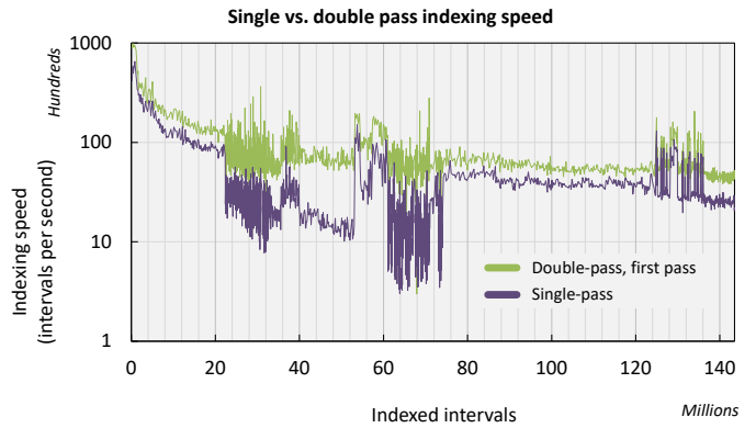
Fig. 10: Benchmarking single-pass and first pass of double-pass indexing algorithms using A4 dataset.
