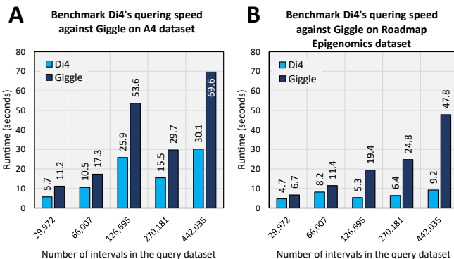
Fig. 7: The runtime plotted here is the average of 10 executions of each query. The results show that Di4 runs up to 3× faster than Giggle on a large dataset (panel A), and up to 6× faster on a small dataset (panel B).
