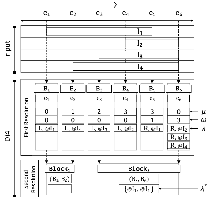
Fig. 13: An example of reconstructing intervals using \lambda^* .
