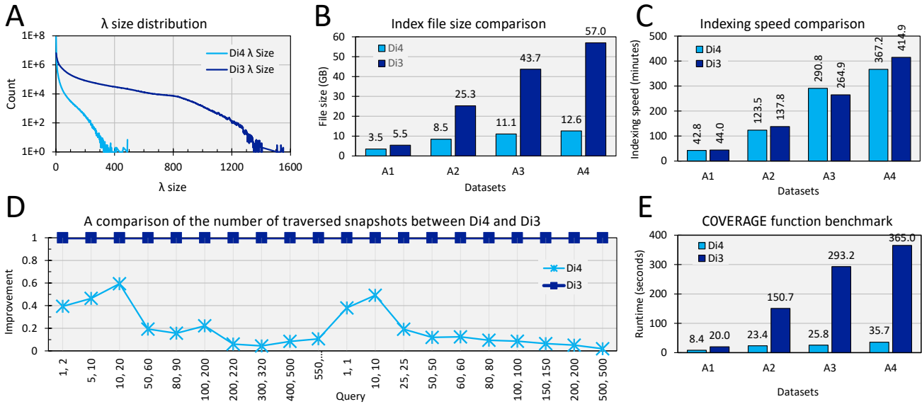
Fig. 5: Panel A compares the \lambda size of Di3 and Di4 when indexing the A4 dataset; it shows that Di4 has significantly smaller \lambda component which results into a considerably smaller index file size, shown in panel B. Panel C shows Di4 indexing speed is comparable to Di3 (both running a double-pass indexing method). The secondary resolutions of Di4 heuristically minimize the number of snapshots to be traversed when executing a query, panel D plots this improvement w.r.t. Di3. As a result of smaller snapshots (panel A), smaller index size (panel B), and heuristically improved query execution (panel D), Di4 runs significantly faster than Di3 (panel E).
