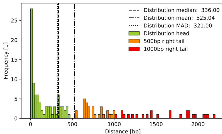
Figure 5: Distance distribution inferred from minimal distance couples of transcription factors CTF and JUN in cell link HepG2. Vertical lines denote statistical aggregators used in TICA tests (mean, median and median absolute deviation). Two dimension for the right tail are given: long (distance greater than 500bp, orange) and short (distance greater than 1000bp, red). Right tail size in this case is approximately 15% of the total.
