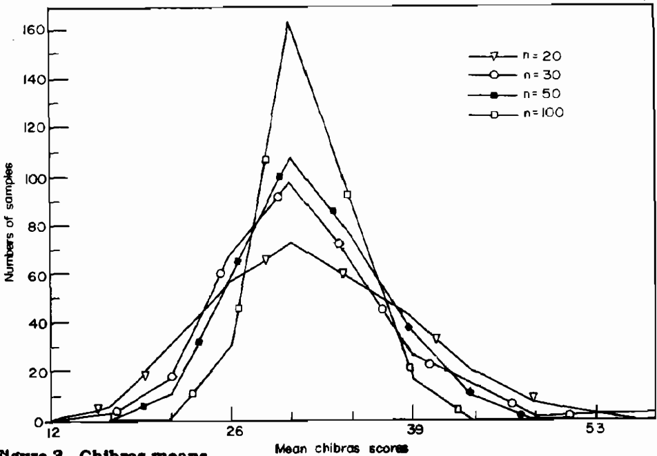
Figure 3. Chibras means
