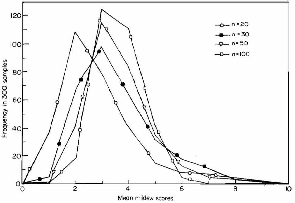
Figure 4. Mildew means
