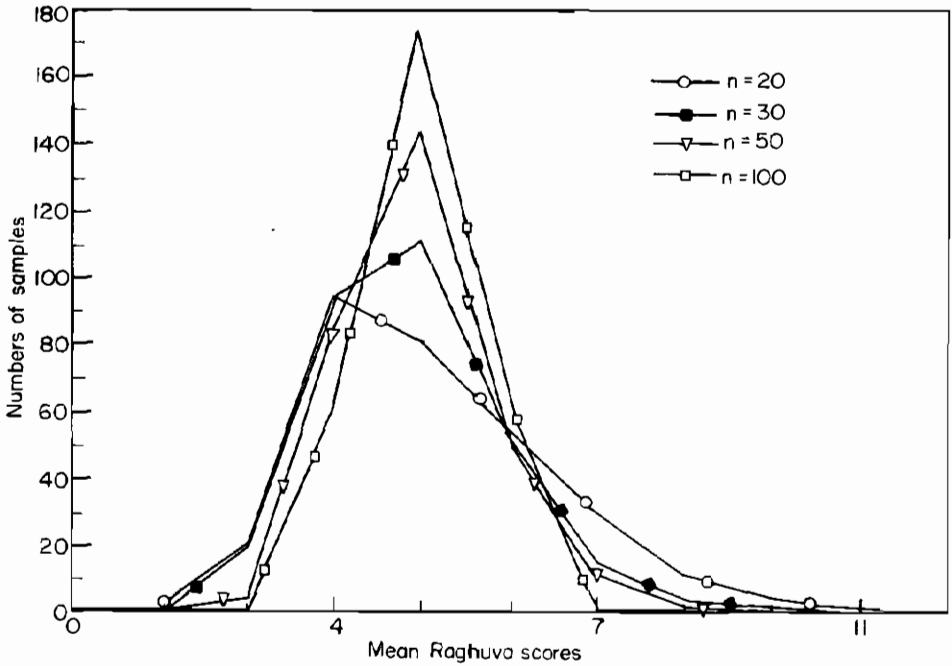
Figure 5. Raghuva means
