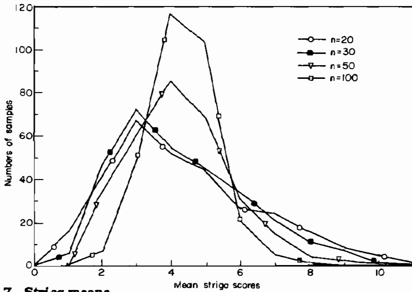
Figure 7. Striga means
