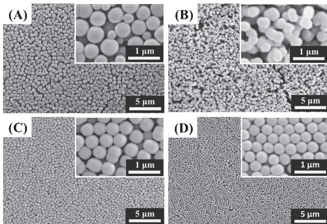
Fig. 2 SEM photomicrographs of titanium glycolate sphere powders synthesized using different concentrations of surfactant: (A) 0 \mu\text{L} , (B) 5 \mu\text{L} , (C) 10 \mu\text{L} , and (D) 20 \mu\text{L} .
