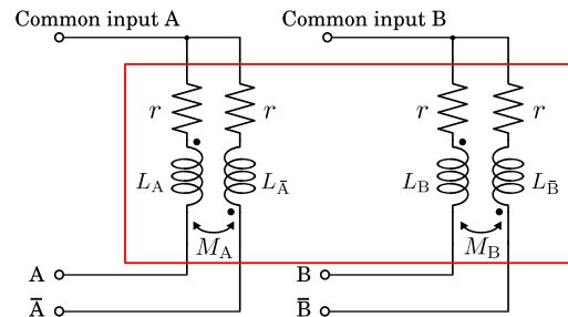
Figure 5: Electrical circuit diagram of a stepper motor.
