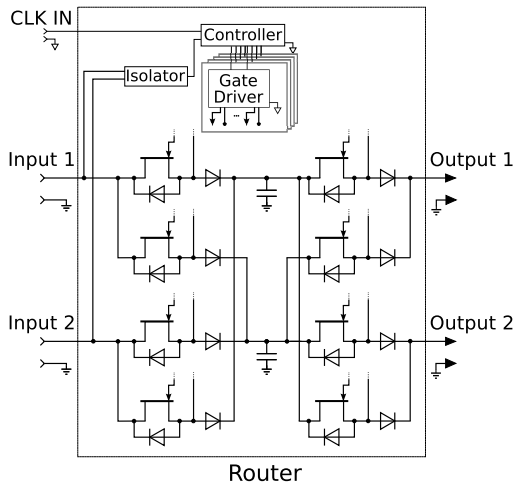
Figure 3: Configuration of power router.
