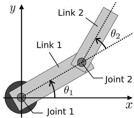
Figure 4: Configuration of 2 DOF manipulator.
