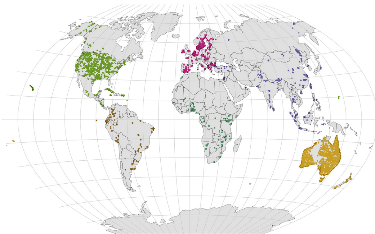
Fig. 3. Locations of the 12 509 unique sites with reflectance spectra that are in the global database.
