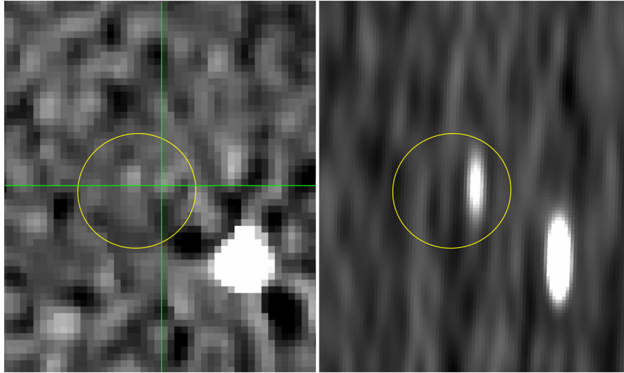
Figure 2. Right: a steep spectrum pulsar candidate towards 3FGL J1639.4–5146 with a high likelihood ratio ( \Lambda ) in the centre of the TGSS ADR image at 150 MHz (175 mJy) shown here with the original Fermi error ellipse (yellow line). On the left is a SUMSS image at 843 MHz with (green) cross-hairs indicating a faint, uncatalogued radio source ( <3 mJy) at the same position as the 150 MHz source. The field of view is 11.9 \text{ arcmin} \times 9.2 \text{ arcmin} and the rms noise in the SUMSS and TGSS ADR images are 1.3 and 9.8 \text{ mJy beam}^{-1} , respectively.
