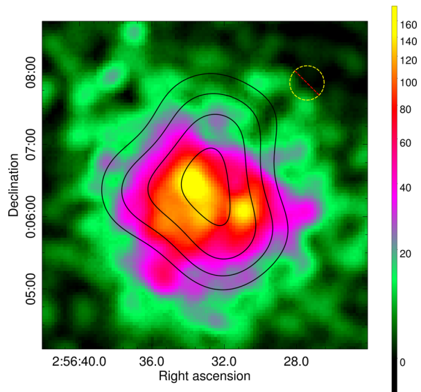
Figure 8. Combined 0.5-2.0 keV MOS1+MOS2 XMM-Newton image of ACT-CL J0256.5+0006 with the 610 MHz radio halo contours overlaid. The contours start at 3\sigma = 0.001 \text{ Jy beam}^{-1} , and increase in steps of 1\sigma . The X-ray image has been exposure-corrected and background-subtracted. The region masked after removing point sources is indicated by the yellow, dashed, excluded circle. The image is unbinned and has been smoothed by a Gaussian with a kernel radius of 6 pixels (1 px = 2.5 arcsec). The units of the colour scale are counts per second per square degree.
