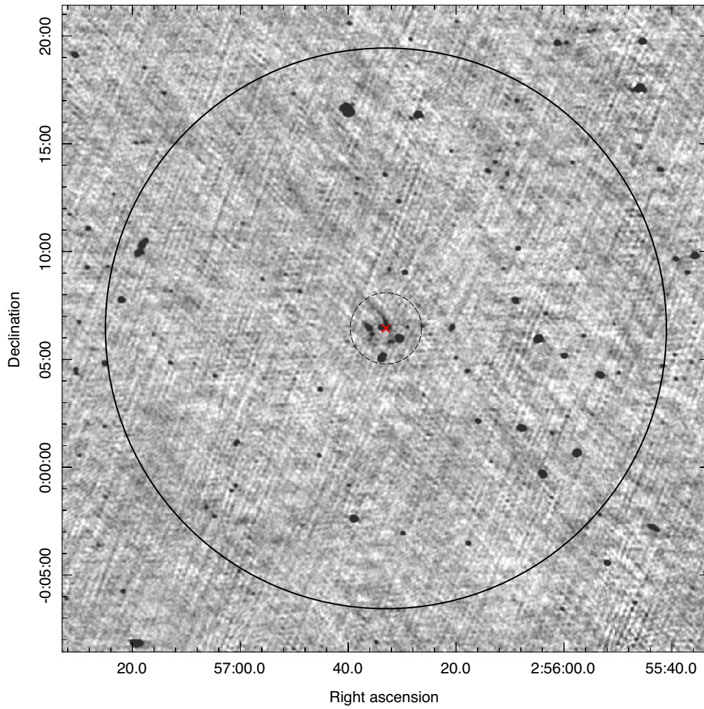
Figure A3. Inner 30 arcmin \times 30 arcmin of the full-resolution (FR) 325 MHz map. The beam is 9.7 arcsec \times 7.9 arcsec at pa 74 ^\circ .1 and the map noise is \sigma = 77 \mu\text{Jy beam}^{-1} . The X and black solid and dashed circles are as in Fig. A1.
