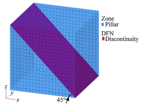
Fig. 4. Discontinuity in the pillar.
