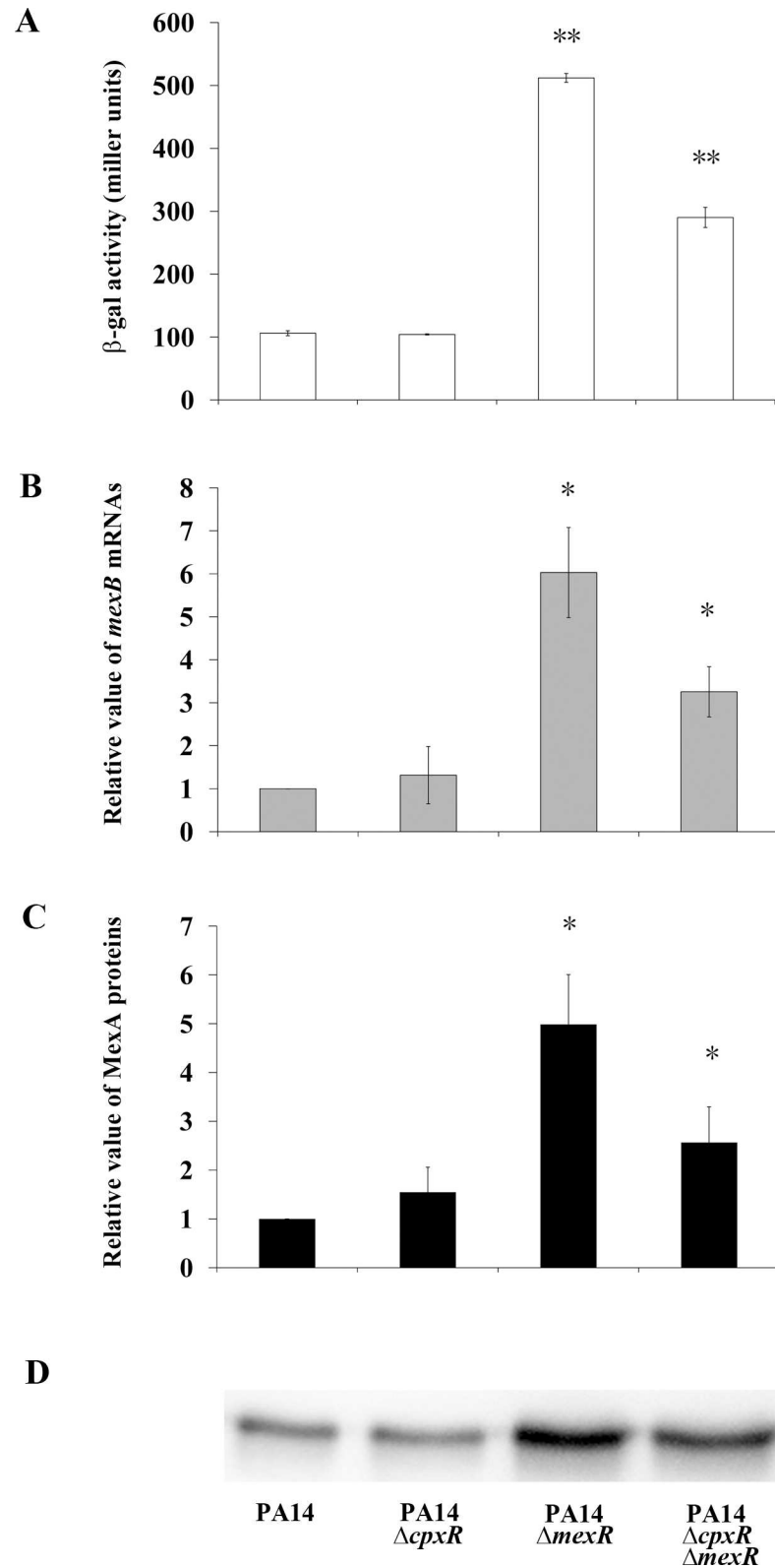
Fig 3. CpxR-mediated up-regulation of mexAB-oprM expression in mexR -deleted P. aeruginosa PA14. (A) The expression levels of mexAp::lacZ reporter as measured by β-galactosidase assay in the PA14, PA14ΔcpxR, PA14ΔmexR, and PA14ΔcpxRΔmexR strains. Each bar represents the mean ± SD of
