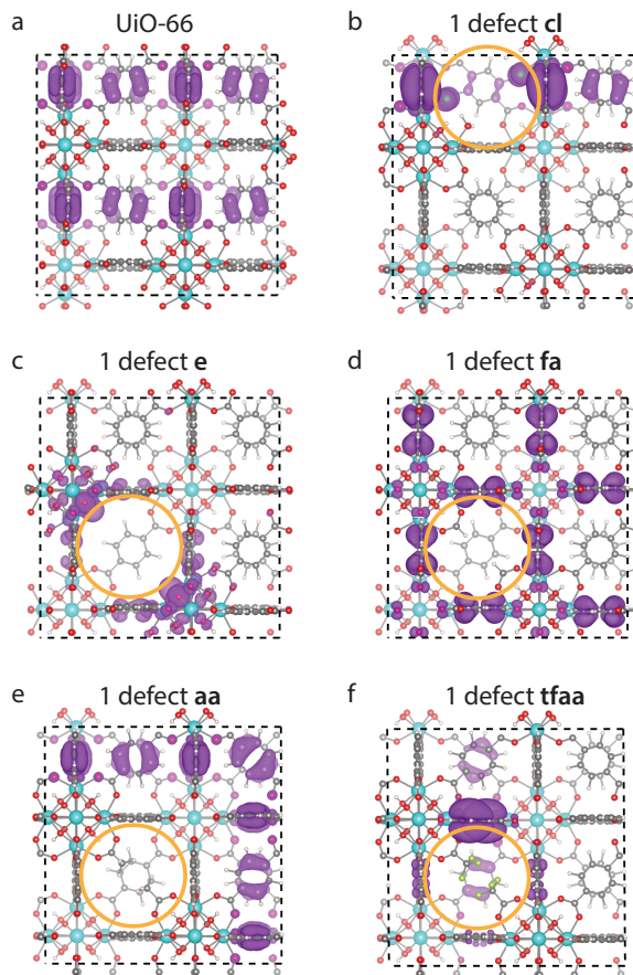
Fig. 5 Electron density of the highest occupied band of a) perfect UiO-66 (top) and UiO-66 with one defect capped by b) cl , c) e , d) fa , e) aa and f) tfaa . The site of the defect is marked by an orange ring, and the isosurface value is 0.00045e/Bohr 3 for all images.
