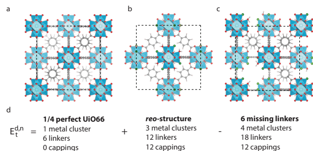
Fig. 1 a) Structure of defect-free UiO-66, b) reo -structure containing missing metal cluster defects and c) the 9_h structure with 6 missing linker defects. Zr is cyan, C is grey, O is red, H is white and Cl is dark green. d) Scheme for comparing the energy of a structure with 6 missing linker defects and the reo -structure.
