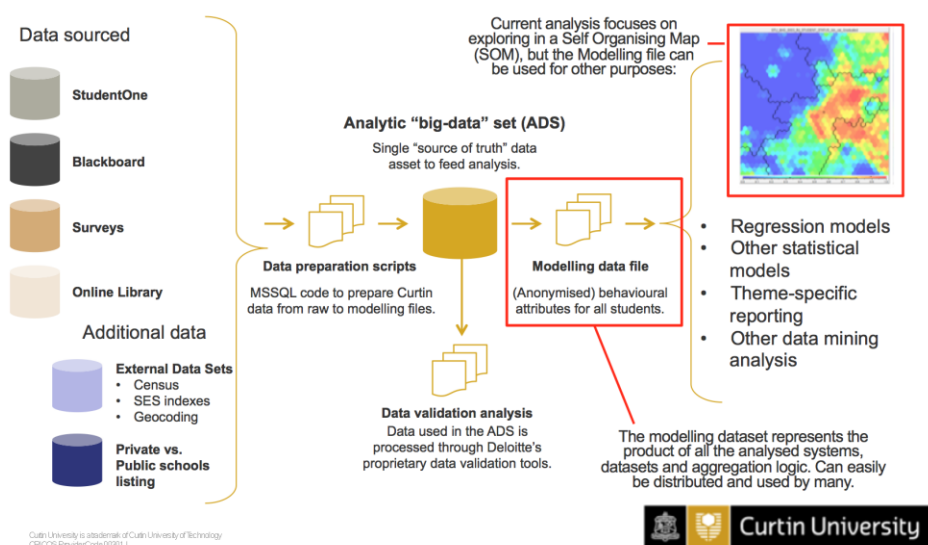
Figure 4. Data sources, analytic data set (ADS) and self-organizing map
