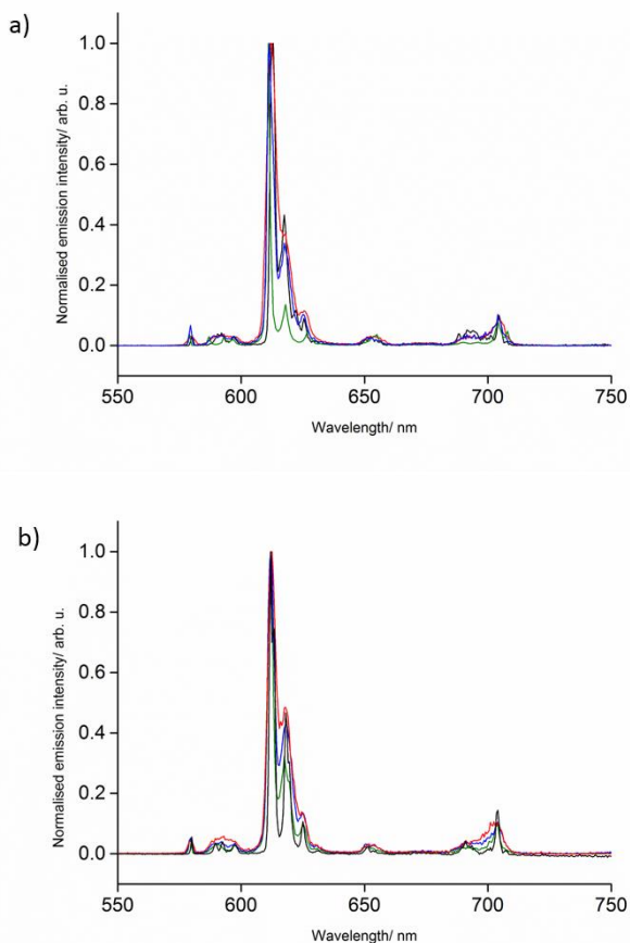
Figure 3 - Normalised emission plots for a) [\text{Eu}(\text{phen})(\text{tbm})_3] and b) [\text{Eu}(\text{phen})(\text{dbm})_3] in solid state (green trace), DCM solution (10-5M) (red trace), 77K (black trace) and PMMA (blue trace), with excitation wavelength at 350 nm.
