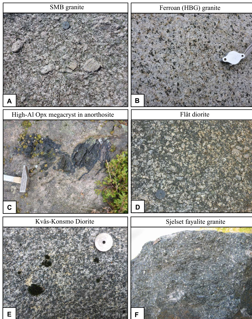
Figure 4. Field photos of Sveconorwegian magmatic rocks. (A) Porphyritic granite from the Sirdal Magmatic Belt (SMB). Coin is 21 mm in diameter. (B) Hornblende-phyric granite from the ferroan hornblende-biotite granite (HBG) suite. Hand lens is ~3 cm across. (C) High-alumina orthopyroxene megacryst from the Egersund-Ogna anorthosite. Hammer head is ~14 cm long. (D) Flåt diorite, Ni-bearing diorite. Coin is 21 mm in diameter. (E) Kvås-Konsmo diorite, intruding the SMB. Coin is 21 mm in diameter. (F) Sjelset fayalite granite. Pencil sharpener for scale; ~2 cm long.
