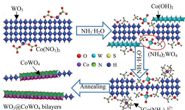
Fig. 3 Schematic illustration of the formation process of \text{WO}_3@CoWO_4 bilayer nanosheets.
