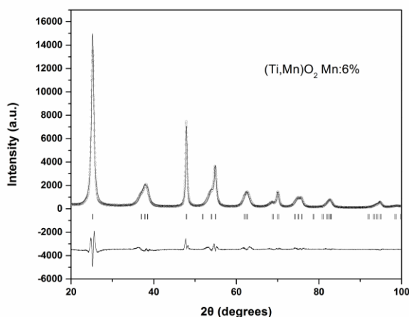
Fig. 2. XRD spectrum of sample 6 at% \text{Mn}^{4+}/\text{TiO}_2 refined by the Rietveld method. (o) experimental points, the continuous line correspond to the calculated spectrum, vertical bars (|) at the bottom indicate the position of Bragg peaks. The continuous line at the bottom is the difference between the experimental intensity values and the calculated one.
