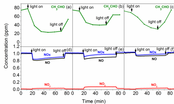
Fig. 7. Concentration profiles of acetaldehyde, NO, NO 2 and NO x gases over the 2 at% Mn 4+ /TiO 2 (a,d), 6 at% Mn 4+ /TiO 2 (b,e), 7 at% Mn 4+ /TiO 2 anatase nanoplates (c,f).
