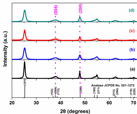
Fig. 1. XRD patterns of the pure TiO 2 (a), 2 at% Mn 4+ /TiO 2 (b), 6 at% Mn 4+ /TiO 2 (c), 7 at% Mn 4+ /TiO 2 anatase nanoplates (d).
