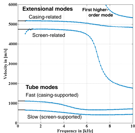
Figure 3: Dispersion curves for an idealized completion model (water-impermeable screen-water-casing-vacuum) when sand screen has vanishing permeability. Note that all modes are completely lossless. Two slowest modes represent tube waves associated with the two fluid columns whereas two fastest modes represent plate (extensional) modes in a screen and casing tubulars respectively.
