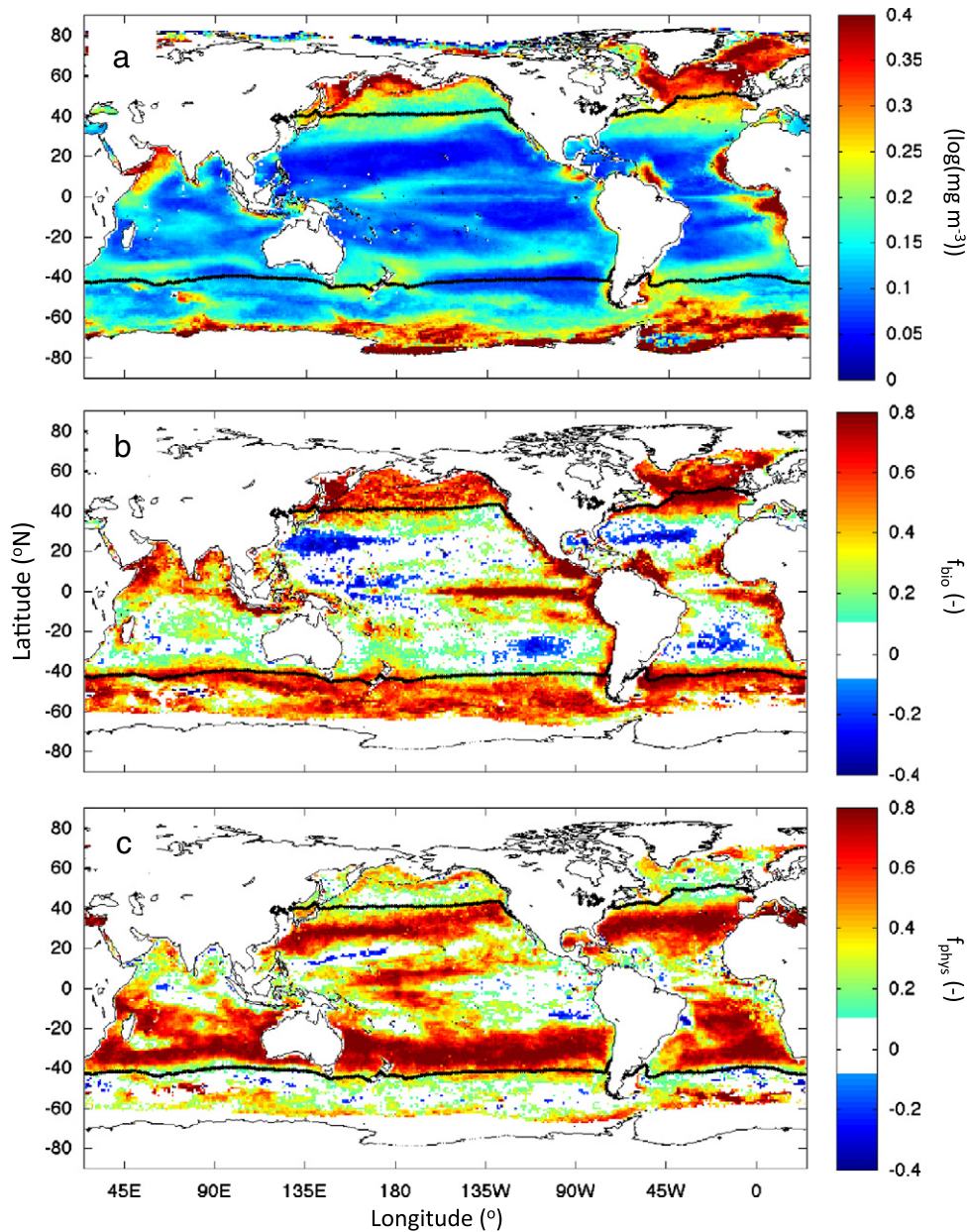
Fig. 8. Chlorophyll variability and its relation to biomass and light-induced physiological changes. a) Standard deviation in \log(\text{Chl}_{\text{GSM}}) estimated over the SeaWiFS mission. b) Standardized regression slopes for predicting \text{Chl}_{\text{GSM}} as function of changes in biomass ( f_{\text{bio}} in Eq. 1) and c) and for changes in rates of photoacclimation ( f_{\text{phys}} ). Values of the standardized regression slopes near one indicate the dominance of that process on \text{Chl}_{\text{GSM}} variability. Details of model configuration are provided in the text. Only statistically significant (95% c.i.) slope values are shown. The mean SST = 15 °C isotherm is shown as the black lines in each panel.
