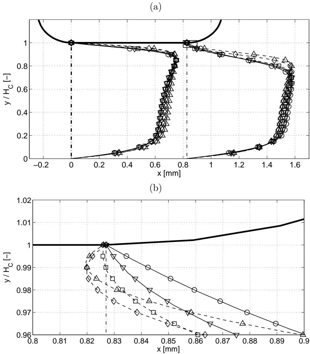
Figure 5. Span-wise profiles of the normalized average stream-wise velocity at the constriction entrance x_{CB} (thick - \cdot - ) and exit x_{CE} (thin - \cdot - ) for the five aperture ratios H_C/H considered, 30% ( \Delta ), 20% ( \diamond ), 10% ( \square ), 8% ( \nabla ) and 6% ( \circ ). (b) is a zoom on the region indicated on (a). The teeth-shaped obstacle wall is indicated with thick — .
