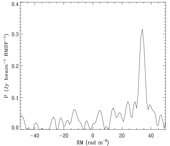
Figure 4. Faraday depth spectrum of PMN J0351-2744 at 189 MHz. The spectrum peaks at \phi = +34 \pm 2 \text{rad m}^{-2} . The uncertainty is dominated by ionospheric Faraday rotation fluctuations.
