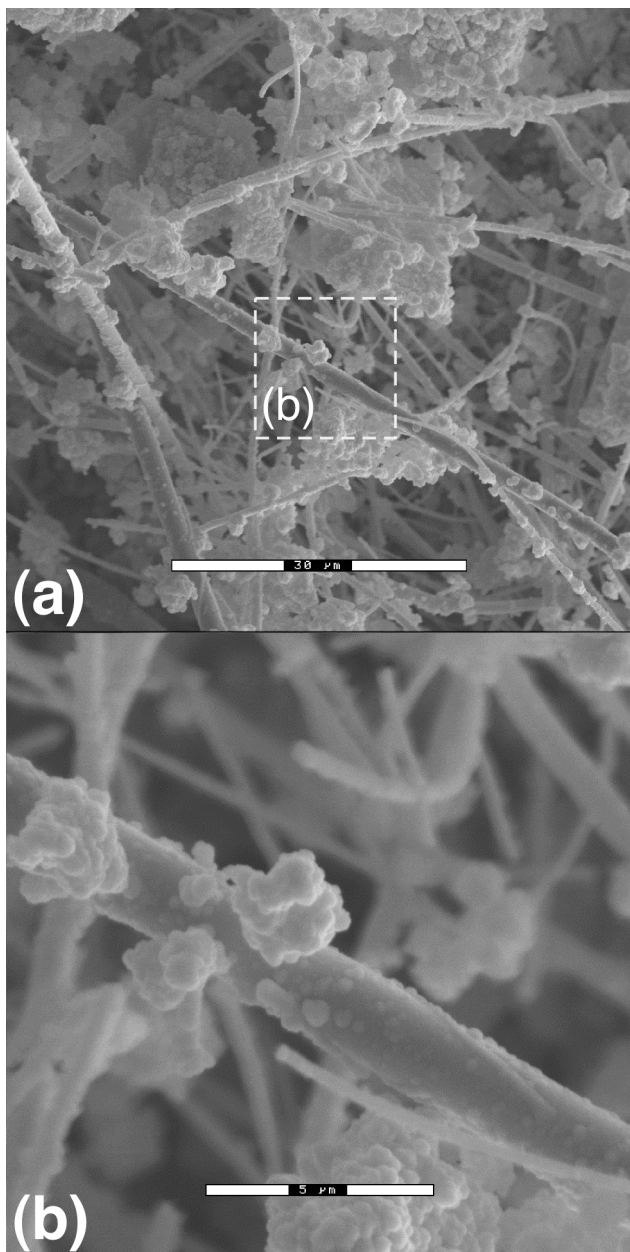
Figure 6 Scanning electron micrographs of NCS (NCS-2EE) after reaction with 0.1 M \text{H}_2\text{PO}_4^- for 24 hours at 25 °C at increasing magnification
