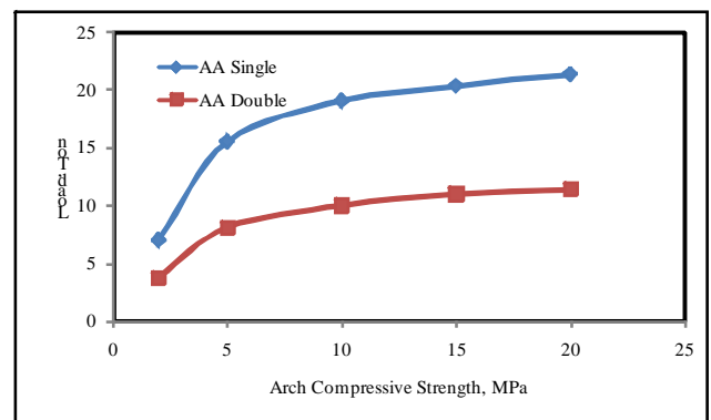
Fig. 9 The effect of arch compressive strength with constant tensile strength of 0.75MPa, Griffith Bridge
