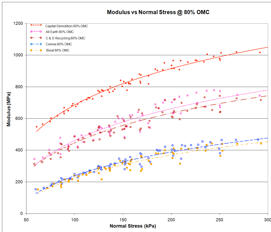
Figure 5: Modulus vs. normal stress for recycled and quarried roadbase materials.
