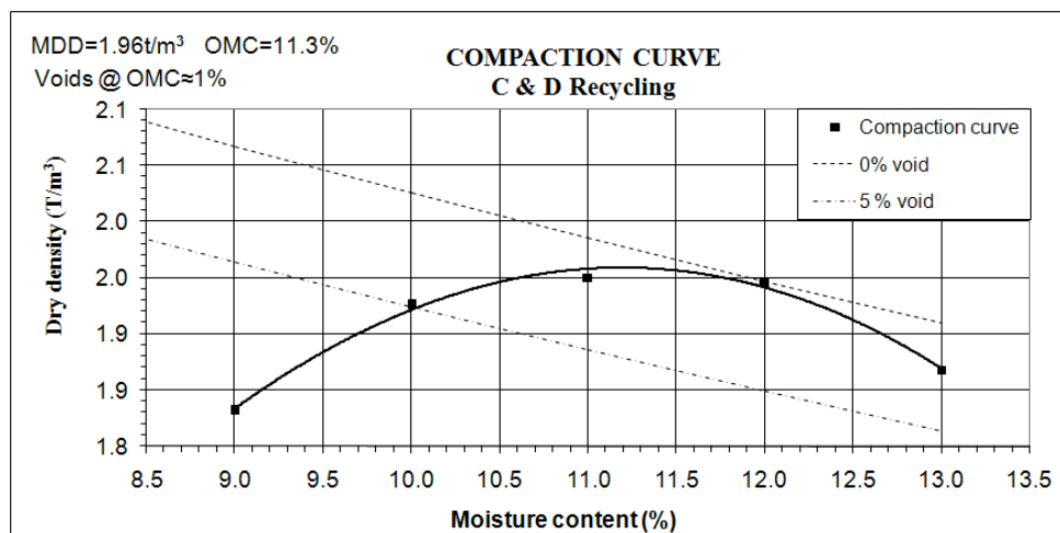
Figure 1: The C & D Recycling compaction curve.
