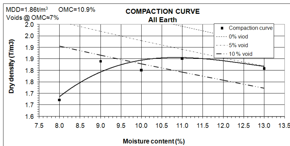
Figure 2: The all Earth compaction curve.
