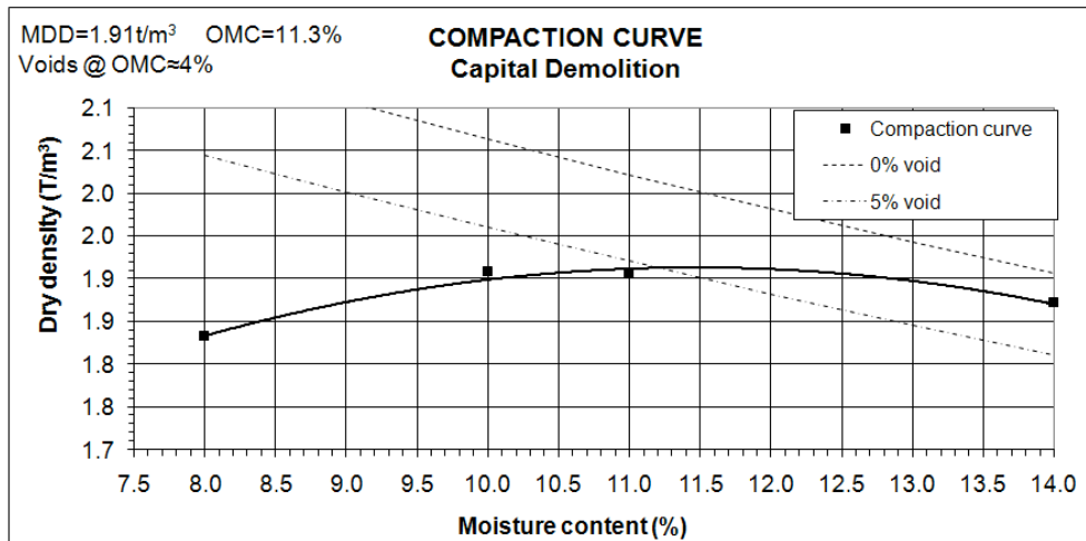
Figure 3: The Capital Demolition compaction curve.
