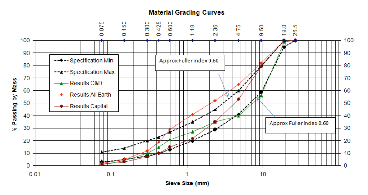
Figure 4: Particle size distributions for recycled materials.
