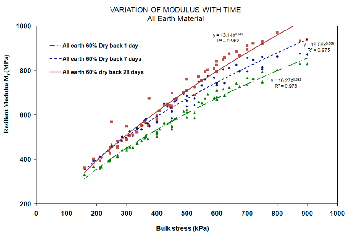
Figure 6: The All Earth resilient modulus at 1, 7 and 28 days.
