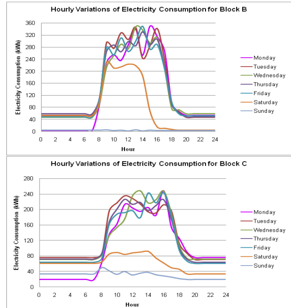
Fig. 6 Week One Electricity Consumption Hourly Variations
