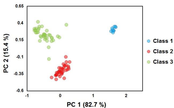
Fig. 3 Two-dimensional PCA scores plot showing distribution of cling film samples into three distinct classes based on their infrared spectral properties
