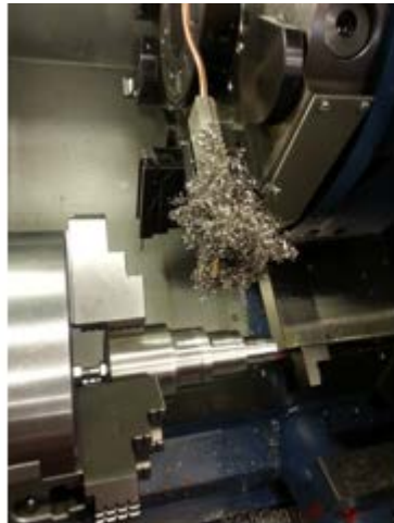
Figure 9. MQL cooling encouraging poor chip breaking at higher cutting speed.
