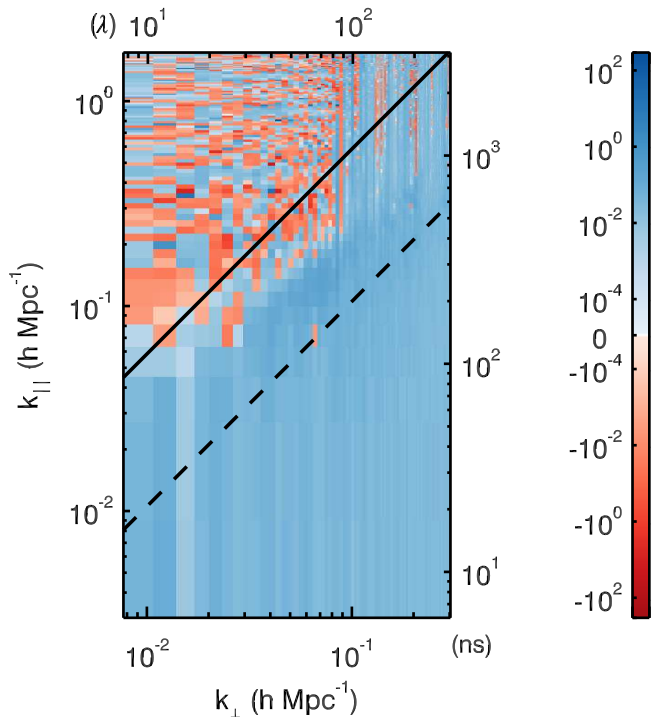
Figure 7. Power spectrum ratio difference, according to Equation 6. This metric shows the difference in the fractional E-W residual 2D power spectrum, comparing the MWACS catalog and our hierarchical catalog. By dividing the residual spectrum by the corresponding dirty spectrum before subtracting we remove the effect of the overall flux scale change due to differing calibration solutions. We see that the wedge is completely positive (higher fractional residual when using the MWACS catalog), confirming that the hierarchical catalog subtracts more power from the data. This also reassures that the calibration using the new catalog is more accurate.
