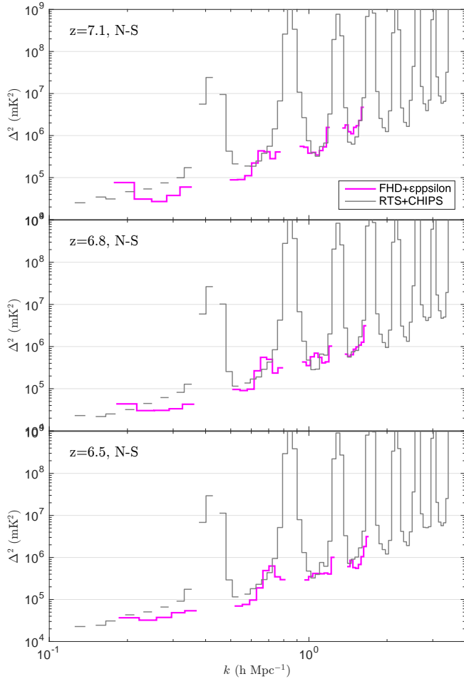
Figure 16. Here we compare the upper limits from the FHD+ \epsilon pipeline with those from the RTS+CHIPS pipeline. The magenta lines are repeated from Figure 15, and the gray lines are the power plus two sigma thermal error bars generated by CHIPS. Due to the logarithmic binning used by CHIPS, some bins are empty, resulting in gaps in the spectra. CHIPS does not excise the coarse band harmonic lines, and so we see their strong effect where there are gaps in the magenta lines. The RTS+CHIPS pipeline accesses larger k modes because the data is processed at 80 kHz, whereas the FHD+ \epsilon pipeline averages to 160 kHz when gridding. The most notable differences are the ability of the RTS+CHIPS pipe to access lower k modes, while the FHD+ \epsilon pipe suppresses more power before and after the first coarse band harmonic. While the different analysis methods result in slightly different upper limits, they are generally in agreement.
