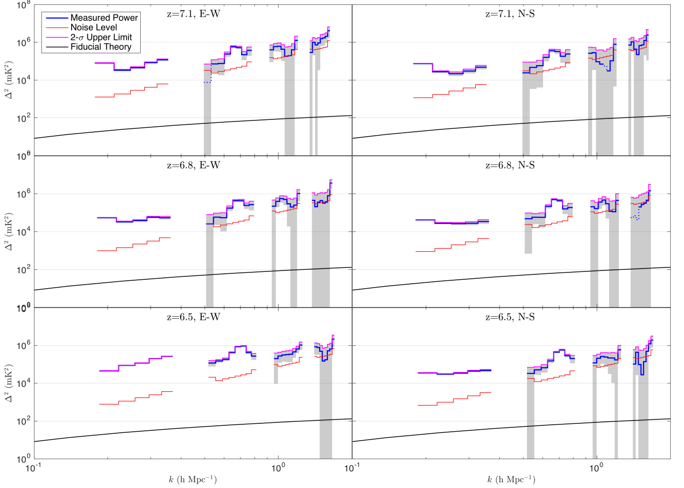
Figure 15. One dimensional power spectra for our three sub-bands and both instrumental polarizations. The solid blue line shows the measured power spectrum with step widths corresponding to the bin size used in the average. Where the measured signal is negative we plot the absolute value with a dotted line. The gray boxes show the \pm 2\sigma error bars on the measured power spectrum. Where the boxes meet the horizontal axis we are consistent with zero. The thin red line is the 1\text{-}\sigma noise level, and the magenta line is the 2\text{-}\sigma upper limit for each k bin. A fiducial theoretical model for a fully neutral IGM from Furlanetto et al. (2006) is shown in black for reference.
