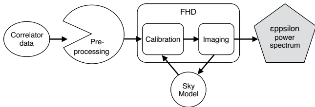
Figure 1. Schematic of the analysis pipeline used in this work. The raw correlator data is preprocessed by performing RFI and other flagging. Then the data are calibrated and imaged using an iterative foreground modeling approach with the FHD package. Finally, a power spectrum is formed using the \epsilon ppsilong package.
