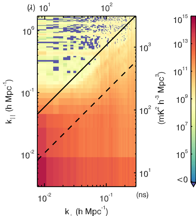
Figure 2. An example two dimensional, E-W polarization residual power spectrum formed using the three hour golden data set from August 23, 2013. The foreground wedge dominates the region below the solid black horizon line, while regions above are mostly noise-like with the exception of horizontal coarse band harmonic lines. The vertical streaks at high k_{\parallel} and high k_{\perp} are due to sparse (u, v) sampling beyond the dense core of the MWA. The right axis shows the delay (Fourier dual to frequency) corresponding to the k_{\parallel} axis, and the top axis shows the baseline length (in wavelengths) corresponding to the k_{\perp} axis.
