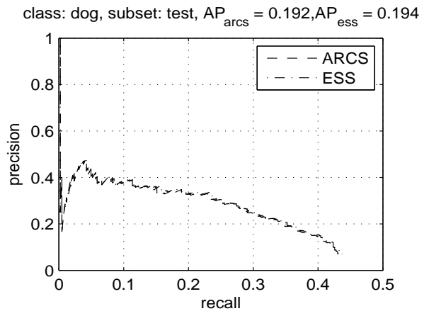
Figure 2. Performance Comparison of the Sub-Images Detected by ARCS and ESS on the Test Images for dog. ESS guarantees global optimization. Though ARCS can not guarantee the global optimization, the performance loss is negligible.
