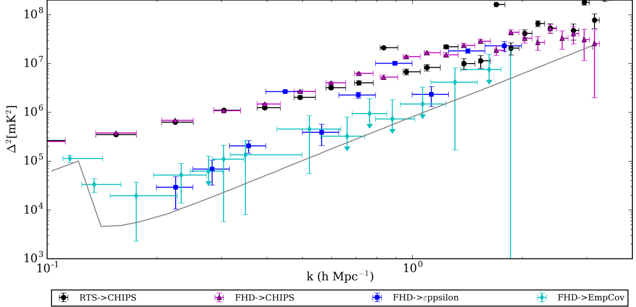
Figure 7. Power spectra averaged along shells of constant k with 2\sigma errors. In three hours of data, four different methods demonstrate different kinds of limits on the power spectrum. Note that of the four pathways shown in Figure 4, only three are included here, but we have now included the EmpCov power spectrum from Dillon et al. (2015) . \epsilonpsilon power spectra of RTS outputs are not shown because, in the version under test here, RTS did not natively produce image-plane error bars, which are required to correctly average from 2D to 1D. Many of the features visible in the 2D plots are also visible here: the excess in the CHIPS spectra is clearly visible as is a smaller excess in the \epsilonpsilon spectrum. The black line indicates 2\sigma bounds for points dominated by noise. Power levels for typical theoretical models are typically in the 5 to 10 \text{mK}^2 range across these k modes.
