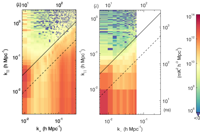
Figure 5. Choice of weighting scheme when applying inverse covariance weights can significantly reduce the effect of the foreground wedge on higher k_{\parallel} modes. On the left, a CHIPS power spectrum where inverse covariance includes a statistical model of confused foregrounds, on the right the EmpCov estimator has weighted by an estimate of covariance formed from the data cube.
