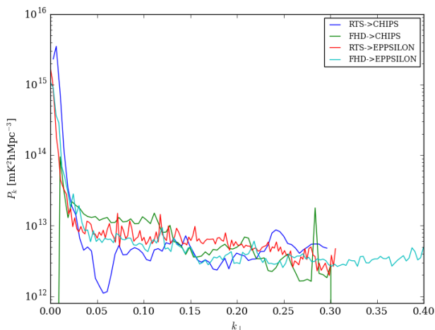
Figure 6. Horizontal cut sampling the k_{\parallel} = 0 mode of the 2D power spectra shown in Figure 4 indicating good agreement on flux scale and foreground power shape over most k modes. The foreground subtraction model only includes point sources. The steep rise is likely due to the bright, smooth galactic foreground emission visible in the residual images in Figure 3 and power spectra by Thyagarajan et al. (2015b). Power spectra produced by EmpCov did not include the k_{\parallel} = 0 mode.
