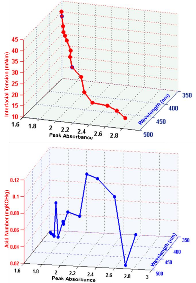
Figure 3. IFT and acid number as functions of peak absorbance and the longest wavelength at which absorbance could be detected.
