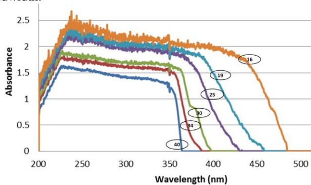
Figure 2. UV-Vis absorbance spectra for various oil samples. The encircled numbers are the corresponding IFT values (in mN/m) [28].
