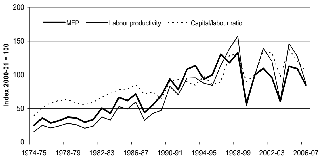
Figure 2.14 Copper ore mining: MFP, labour productivity and capital/labour ratio, 1974-75 to 2006-07
