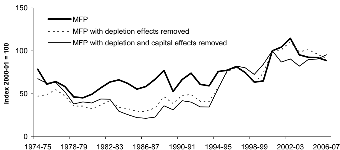
Figure A.14 Other metal ore mining MFP: Impact of resource depletion and capital effects a
