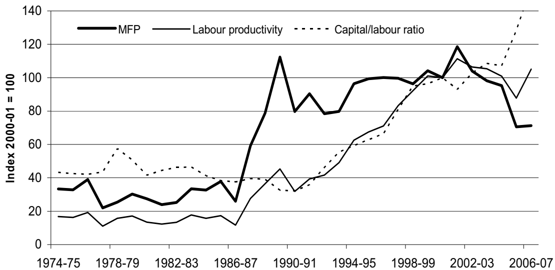
Figure 2.12 Iron ore mining: MFP, labour productivity and capital/labour ratio, 1974-75 to 2006-07
