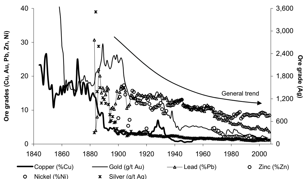
Figure 3.6 Combined average ore grades over time for base and precious metals
