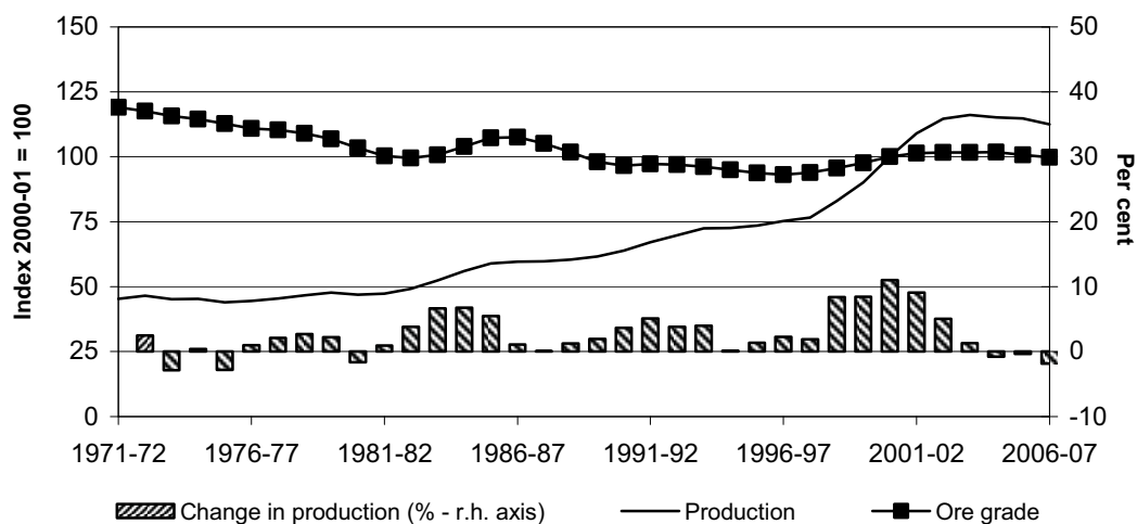
Figure 3.10 Silver/Lead/Zinc ore mining: smoothed production and ore grade, 1971-72 to 2006-07
