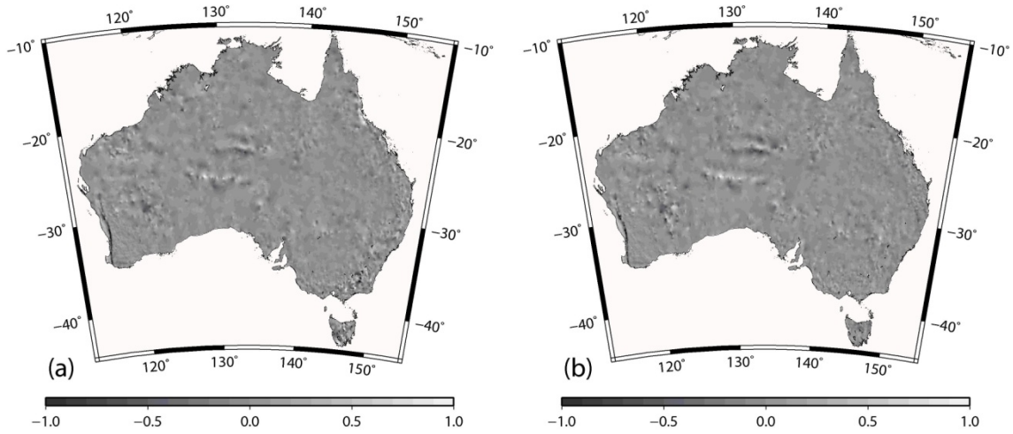
Figure 1: (a) Differences between \delta g_{BM}^{EGM} at \Omega_{BM}^{ANLN} and \Omega_{BM}^{GDA} (maximum 2.1 mGal, minimum -2.33 mGal, RMS \pm 0.2 mGal), and (b) differences between ANGD \Delta g_{SPB} at \Omega_{BM}^{ANLN} and \Omega_{BM}^{GDA} (maximum 1.5 mGal, minimum -2.2 mGal, RMS \pm 0.2 mGal).
