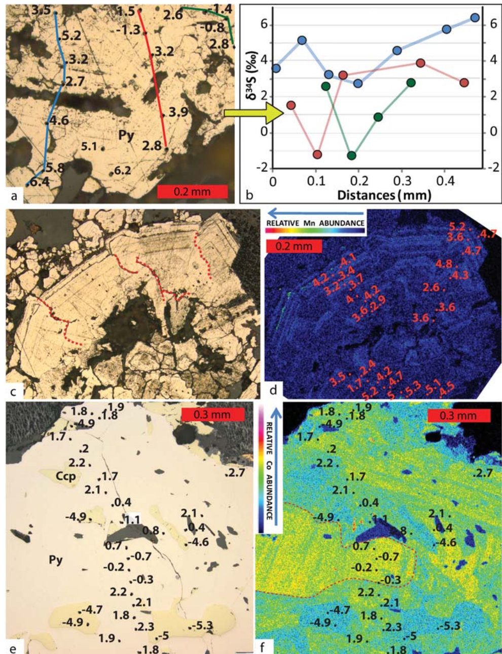
Figure 5. Textures and geochemical features in samples from Beth-Ghinivert. Numbers indicate the measured \delta^{34}\text{S} values. (a) Sample BE51; pyrite aggregate preserving growth textures. (b) The diagram shows the variation of \delta^{34}\text{S} along three transects highlighting the isotopic heterogeneity of pyrite within a few tens of microns. (c) Sample BE51; well-preserved growth textures correspond to a zoned distribution of Mn (shown in Figure 5d). Recrystallization is localized (see red dotted lines indicating boundaries). (d) Sample BE51; relative distribution of Mn in pyrite, mimicking growth textures and evidencing lack of metamorphic rehomogenization of trace elements. (e) Sample BE66; low \delta^{34}\text{S} values occur at the core of this pyrite crystal, whereas higher \delta^{34}\text{S} values occur at the rim. (f) Sample BE66; the distribution of Co evidences relict growth textures. Dotted red lines evidence Co-rich cores (warm colors), which record low \delta^{34}\text{S} values. Oscillation of Co relative concentration is seen at crystal rims where higher \delta^{34}\text{S} values occur.
