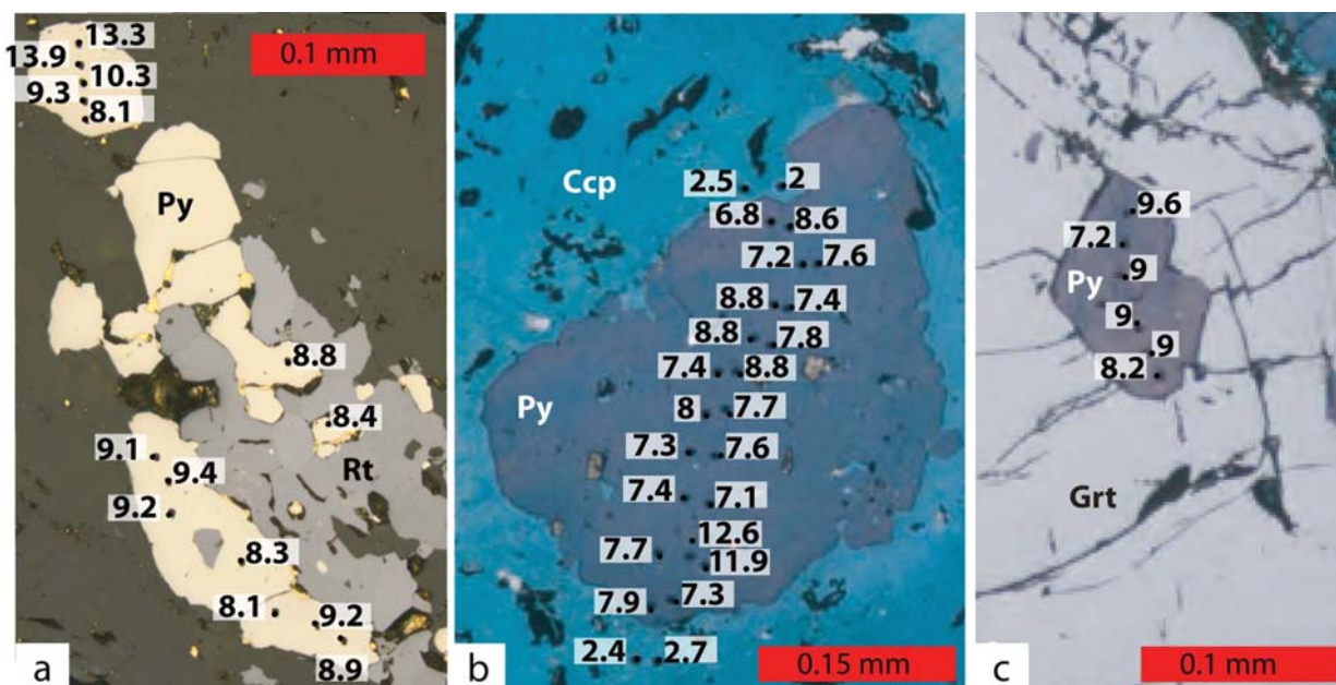
Figure 9. \delta^{34}\text{S} values (‰) in some of the studied samples. (a) Sample SE8 (glauconite); pyrite intergrown with rutile in the metamorphic peak foliation. (b) Sample ATSV-001 (talc schist); pyrite rimmed by chalcopyrite in the matrix. \delta^{34}\text{S} values of the pyrite and chalcopyrite are homogeneous except for two outlying high values in the pyrite. (c) Tiny pyrite inclusions in garnet. ATSV-001. Ccp = chalcopyrite; Py = pyrite; Ru = rutile.
