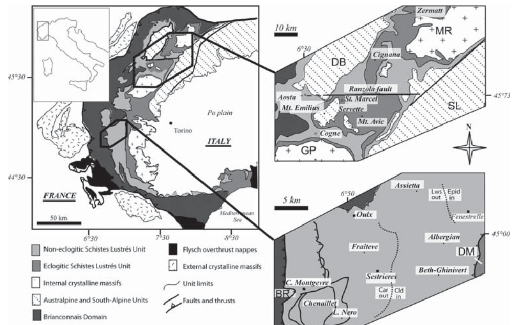
Figure 2. Simplified geological sketch of (left) Western Alps and the detail of the studied zones. (top right) Map of the Servette zone [after Martin et al., 2008]. DB = Dent Blanche Unit; GP = Gran Paradiso nappe; MR = Monte Rosa nappe; SL = Sesia-Lanzo zone. (bottom right) Map of the Beth-Ghinivert zone [after Agard et al., 2001]. BR = Briançonnais Domain; DM = Dora Maira Massif; car = carpholite; cld = chloritoid; Epid = epidote; Law = lawsonite.
