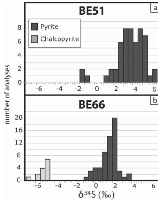
Figure 6. Histograms showing the distribution of \delta^{34}\text{S} values observed in the samples from Beth-Ghivivert. (a) Sample BE51; wide range of \delta^{34}\text{S} values for pyrite. (b) Sample BE66; \delta^{34}\text{S} values for pyrite and chalcopyrite.
