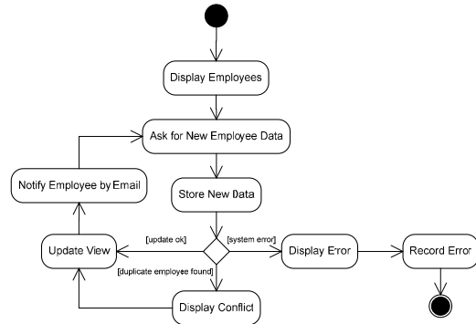
Fig. 4. An updated Activity diagram.
