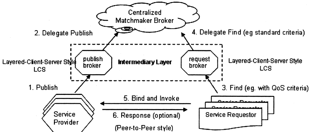
Figure 3. Layered Matchmaker Broker Style
